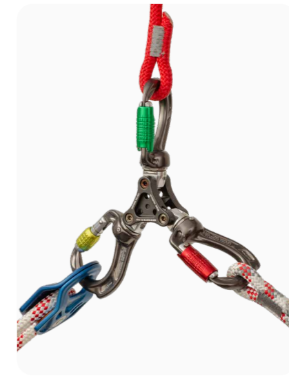
› Three Director Swivel Boss configured with a Linkit Y3 (SW540)
